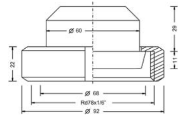
Typ T Tri-Clamp 2"/DN51 PN16/40
